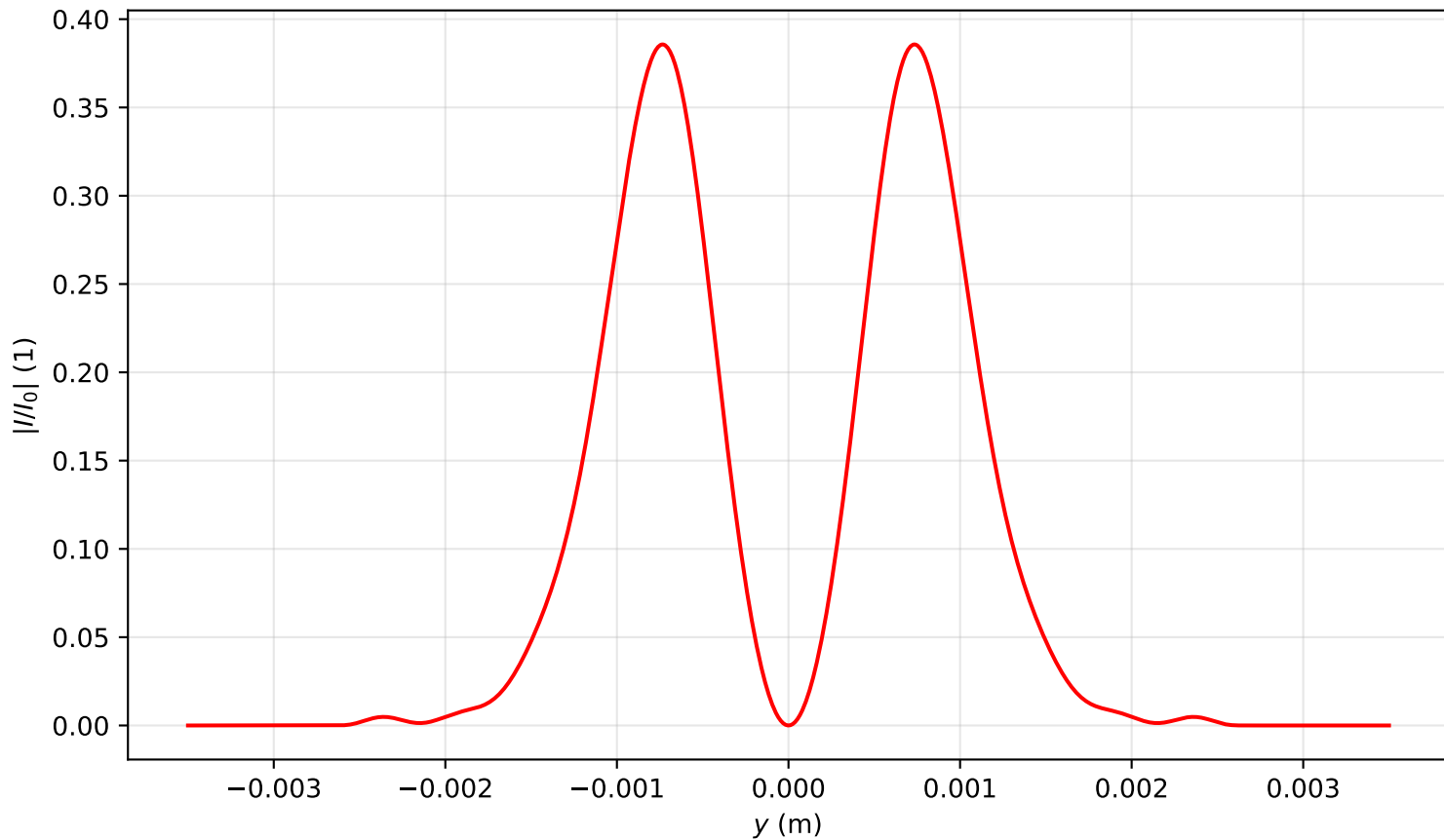
Intensity profile I(x=0, y, z=2.786)/I_0 , P_{in}=3.0P_{cr} , artificial time
